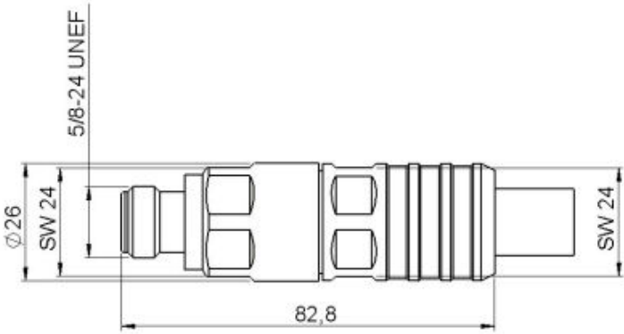
NF-RA12-P02 sketch
