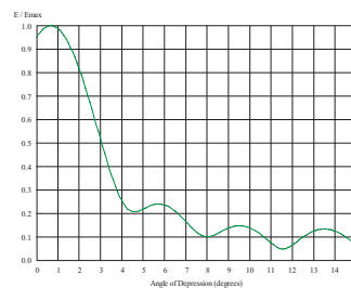
VRP VPOL PCP500-8 12.03dBd
