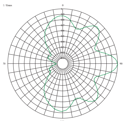
HRP HPOL PCP500-C 3.32dBd
