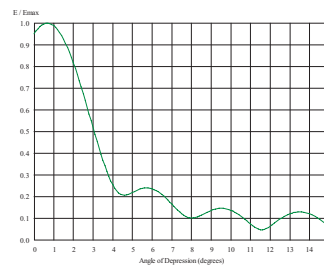
VRP HPOL PCP500-8 12.09dBd
