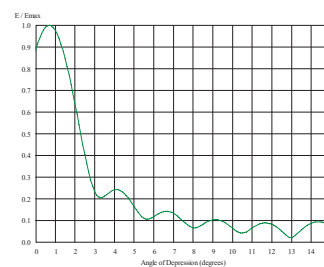
VRP VPOL PCP500-12 13.77dBd
