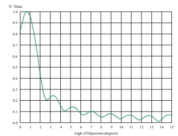
VRP HPOL PCP500-16 15.05dBd
