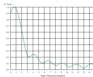
VRP HPOL PCP500-12 13.81dBd
