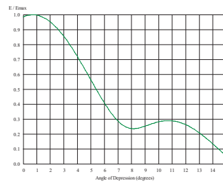
VRP VPOL PCP500-4 9.03dBd
