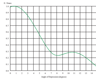
VRP HPOL PCP500-4 9.11dBd
