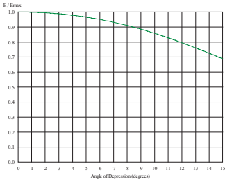
VRP HPOL PCP500-1 3.75dBd
