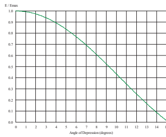
VRP HPOL PCP500-2 6.67dBd
