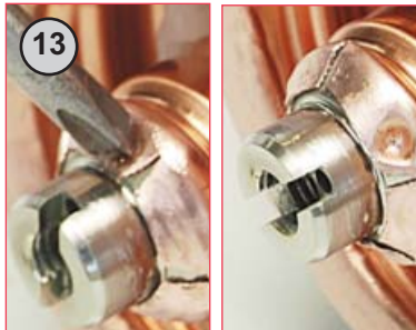
13 Indent cable inner conductor to prevent connector inner nut from rotating.
