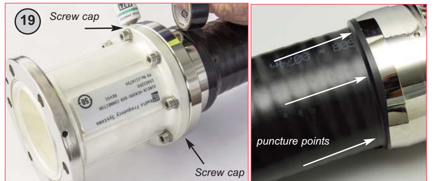
19 Remove both screw caps on back nut. Finely spray back nut/cable with water to accelerate curing. Inject sealing compound (approx 40cc) until the sealant appears at the opposite side of the back nut. Replace cap to stop further flow of sealant. Wrap insulating tape around the rear of the back nut/cable. Puncture the tape in 4 places as shown and then continue injecting compound until it appears at the puncture points. Remove sealant tube cartridge and replace screws. Do not pressurise for 24 hrs to allow compound to harden.
