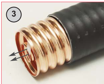
3 Pull out approximately 20mm (3/4") of helix. Trim and discard 12mm (1/2") off the helix then push back into original position. Make sure copper inner & outer edges are smooth and free of burrs and copper surfaces are clean, using the file and scouring pad. Ensure all debris is removed.
