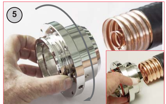
5 Screw connector back nut clockwise as far as possible onto the cable.
