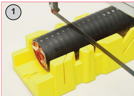
1 Straighten cable and ensure that it is marked and cut square.
