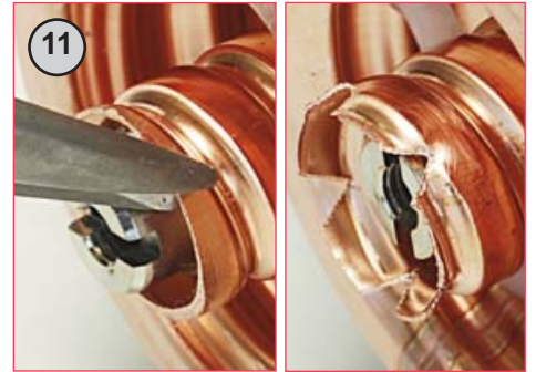
11 Snip inner conductor with 3mm V cuts, approx every 10mm.
