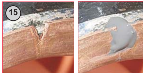
15 In the unlikely event that the outer conductor has split or torn, repair by adding Pactan sealant as shown allowing 45 min to set before fitting the connector body to the back nut.
