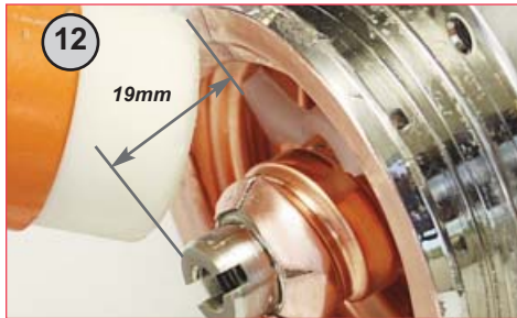
12 Screw inner cable piece out until it protrudes 19mm (3-4") from the outer conductor flared face. Hammer copper to form over inner cable piece. Clean assembly.
