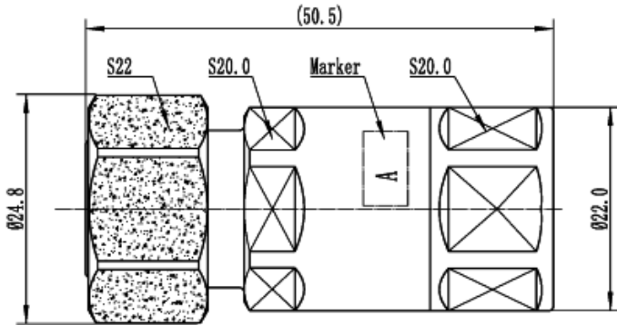
43M-LCF12-C03 Outline Drawing
