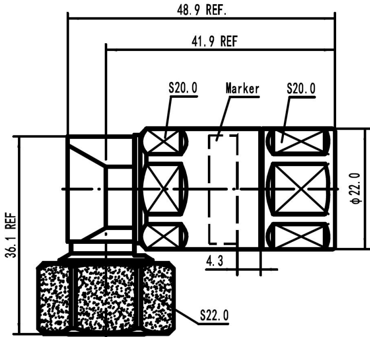
43MR-LCF12-C03 Outline drawing
