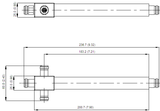
Dimensions mm(inch)
