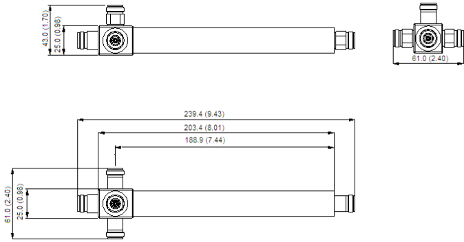
Dimensions mm(inch)
