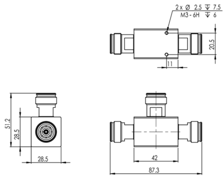
TPS6-43-555_6000_Drawing
