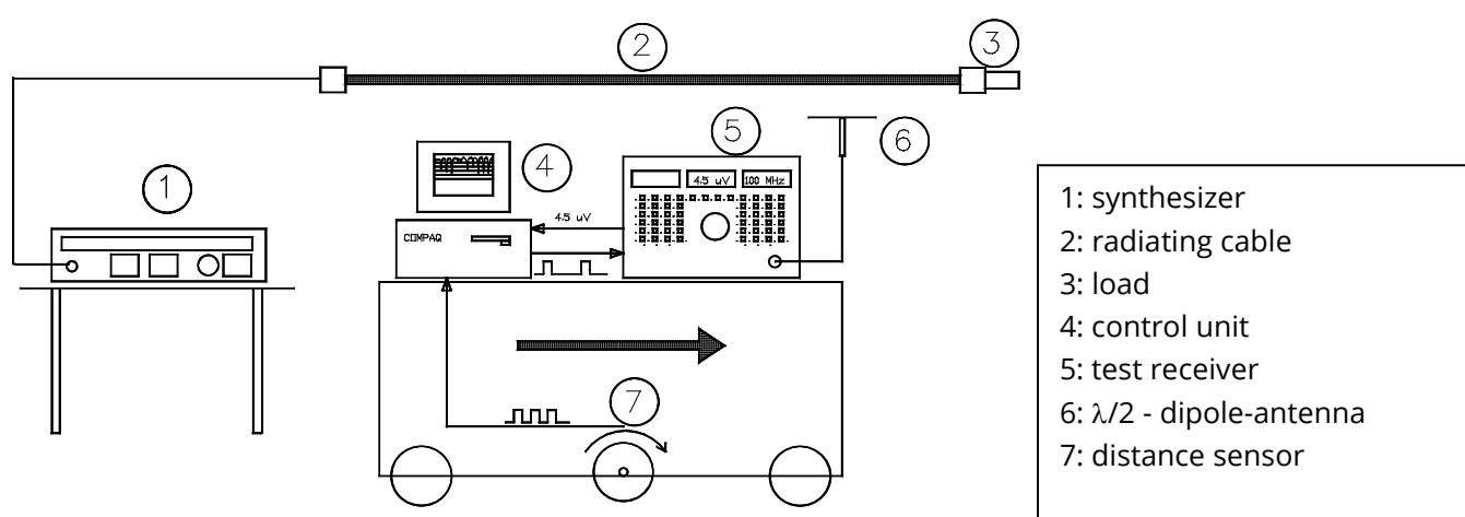
figure 1: measurement equipment
