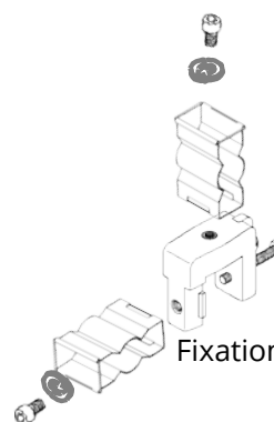
Fixation onto angle-, flat- or U-member with RSB Cleat RSB-310
