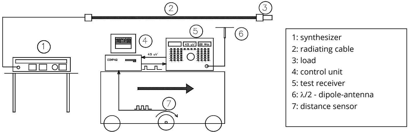
figure 1: measurement equipment
