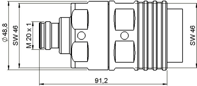
43F-RA114-P02 sketch
