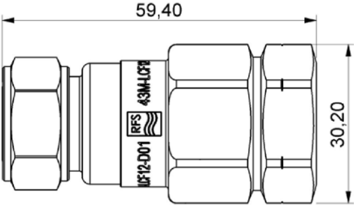
43M-LCF12-D01 Outline Drawing
