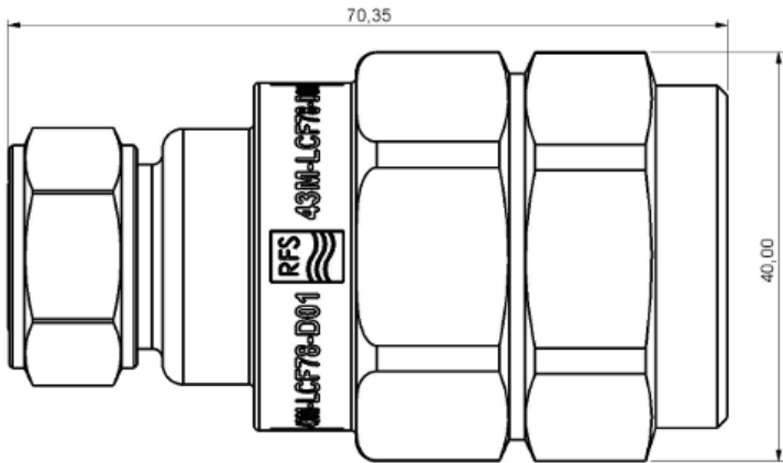
43M-LCF78-D01 Outline Drawing
