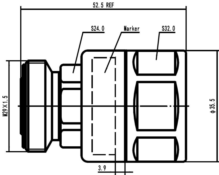
716F-LCF78-C03 Outline drawing
