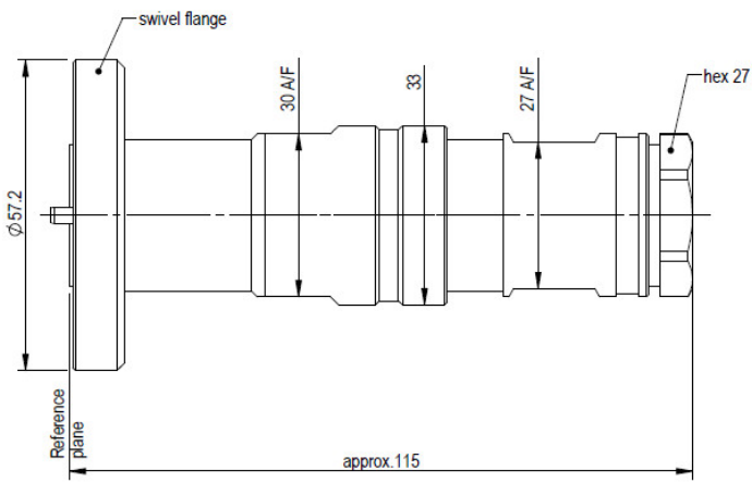
78EIA-HCA58-019 connector, dimensions in mm
