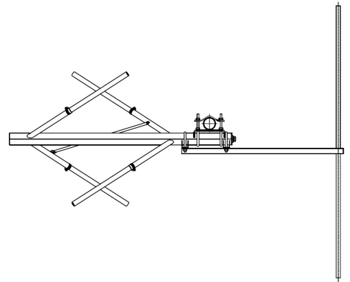
828MPDA antenna (plan view)
