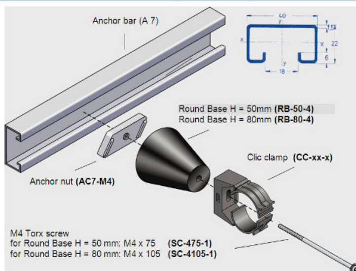
Installation example
