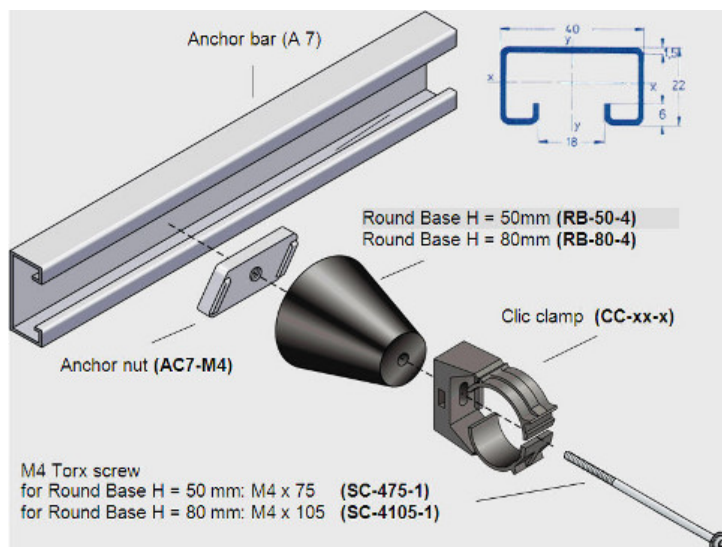
Installation example
