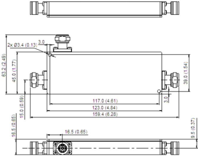
Dimensions mm(inch)
