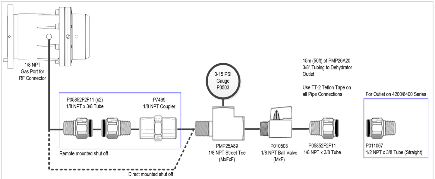
Feeder cable pressurisation - Fittings and Part numbers
