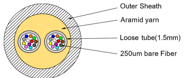
Cable Structure
