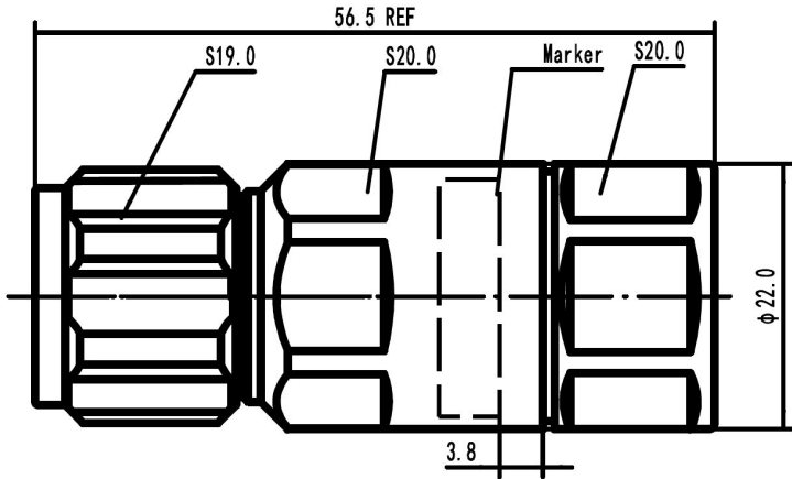
NM-LCF12-C03 Outline Drawing
