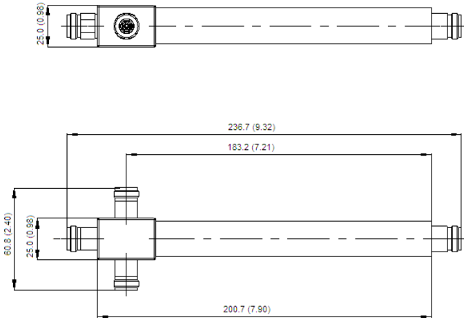
Dimensions mm(inch)
