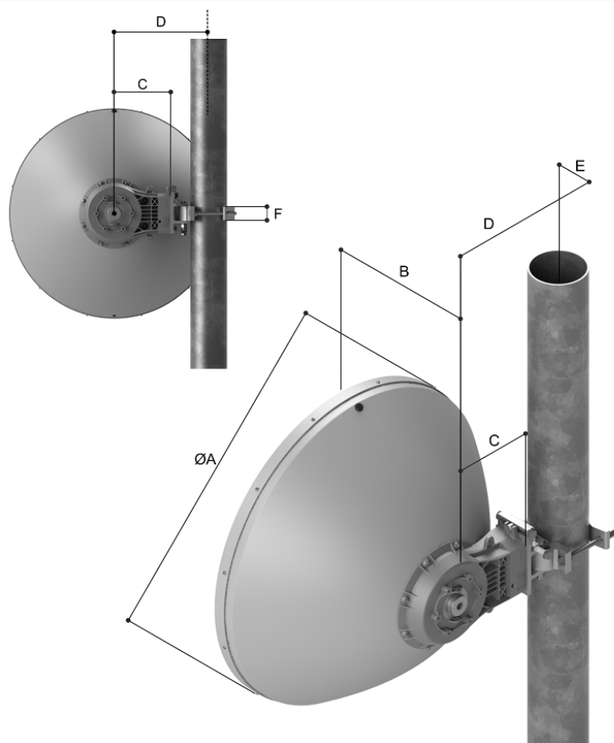
Mount outline
