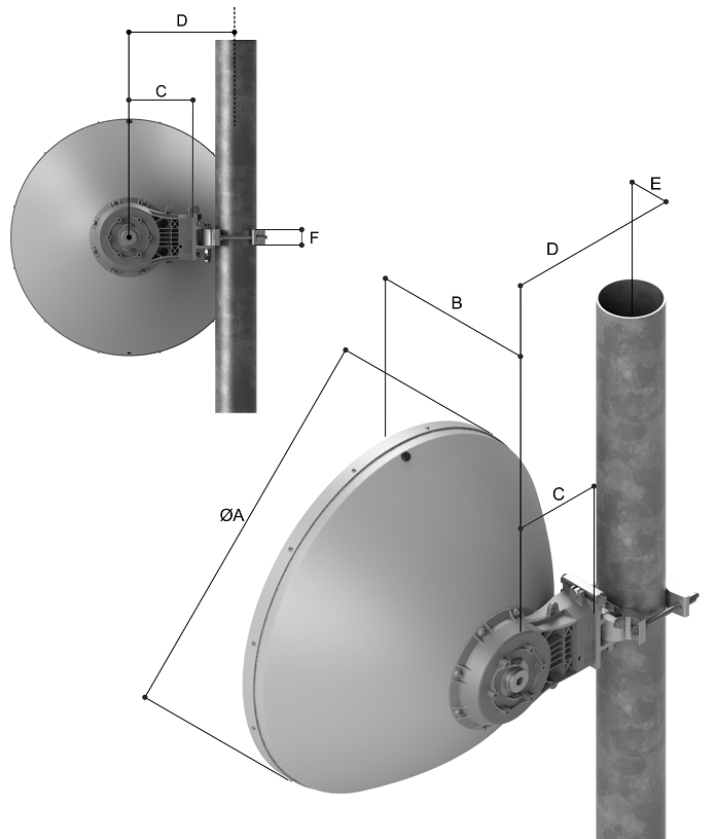
Mount outline
