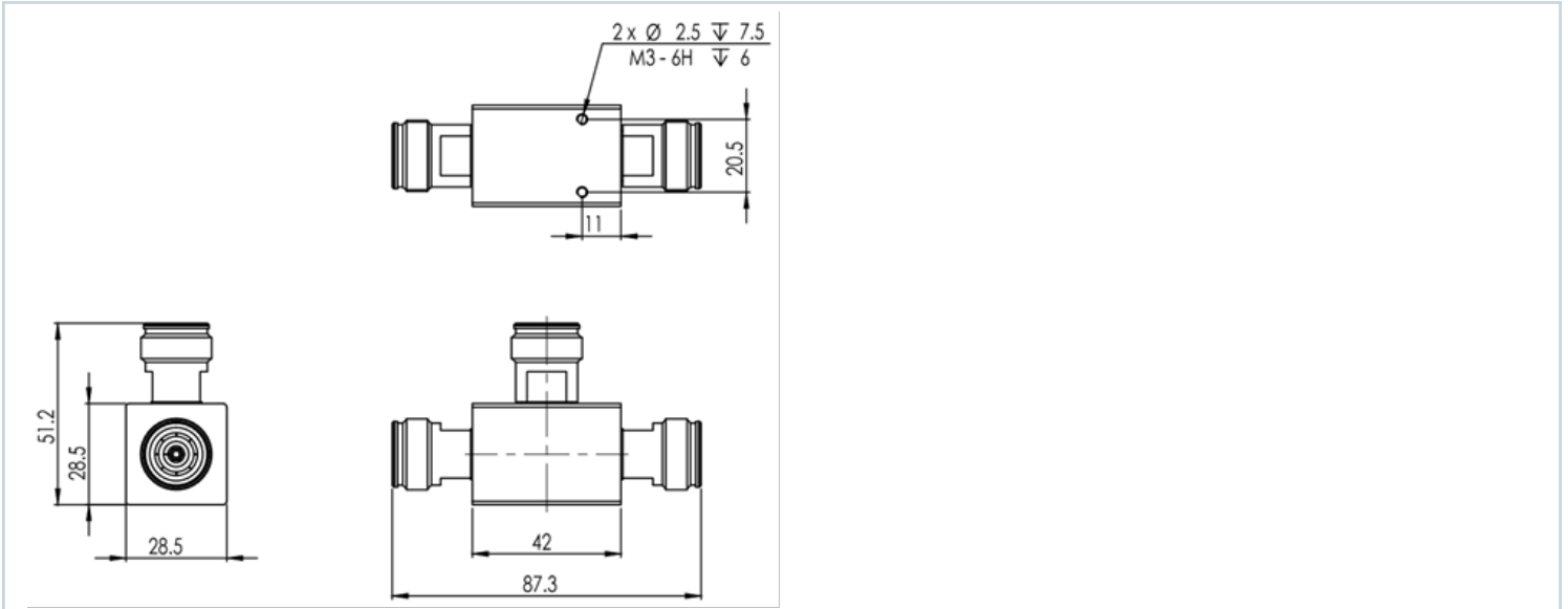
TPS3-43-555_6000_Drawing
