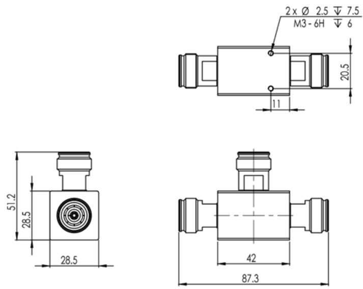
TPS3-43-555_6000_Drawing
