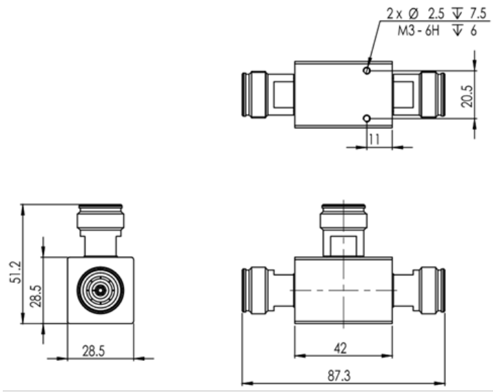
TPS5-43-555_6000_Drawing
