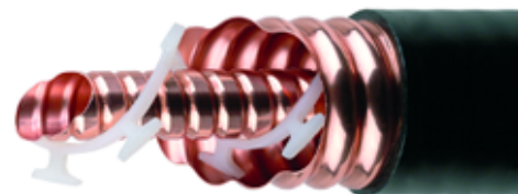
8" HELIFLEX® Air Dielectric Coaxial Cable
