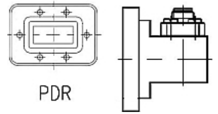
Coax transition for R120 and smaller waveguides
