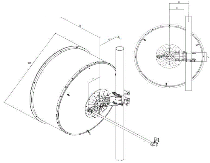
Outline 4ft UXA
