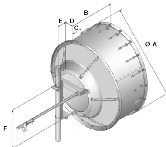
Outline_10ft_High_Perf_Antenna_250
